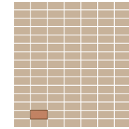
STACK BOND
